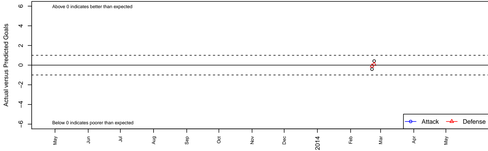
CCV Stars 00 Black G99 Dots are actual minus expected GF (blue circles) and GA (red triangles). Blue line is smoothed change in attack strength. Red is smoothed change in defense strength.
